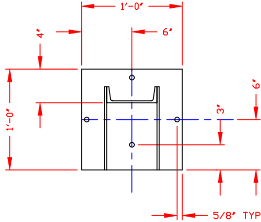
BASEPLATE DETAIL SHOWING CHANNEL & GUSSETS
